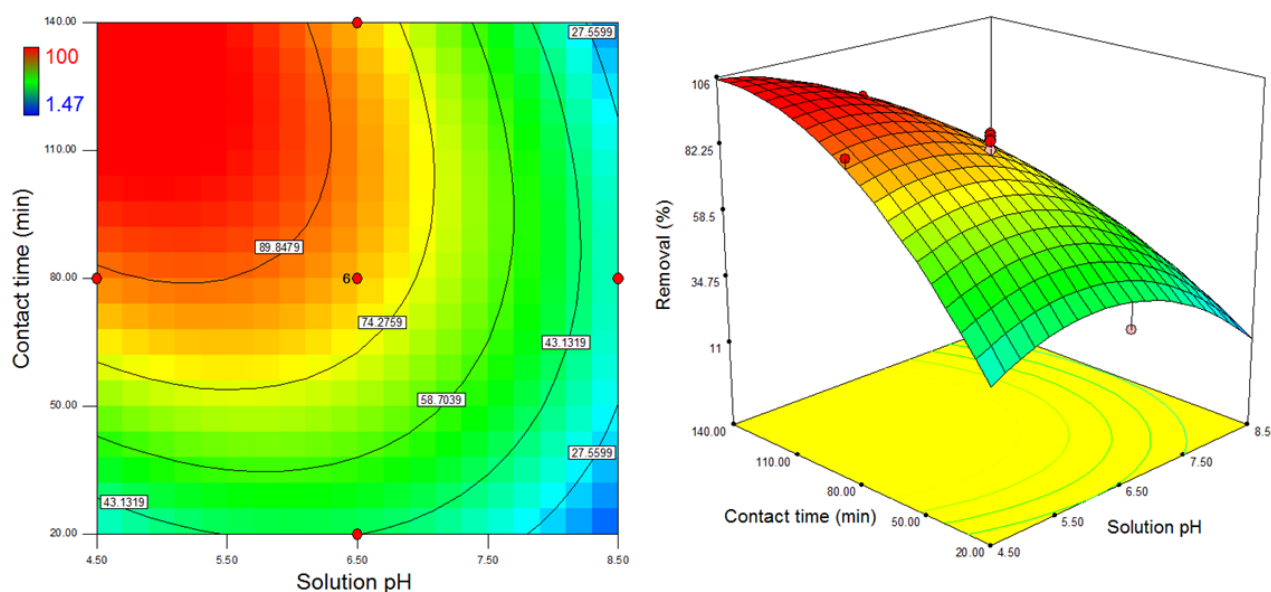
Fig. 6. Two-Dimensional and Three-Dimensional Response Surface Diagrams Depicting the Effects of Solution pH and Reaction Time at the 70 \mu\text{g/L} Arsenate Concentration
