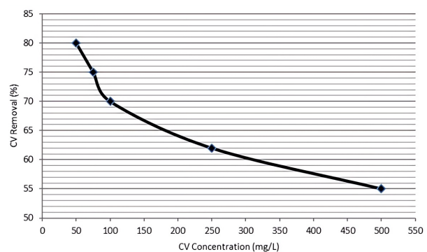
Fig. 9. Effect of The Initial Dye Concentration; (a) CV Initial Concentration of 5-30 mg/L, (b) CV Initial Concentration of 50-500 mg/L
