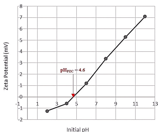
Fig. 3. Identification of \text{pH}_{\text{PZC}} of PHP
